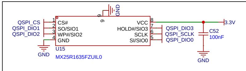
FLASH_MEMORY
